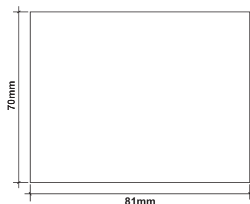
Figure 2.2 Panel Cut-Out
